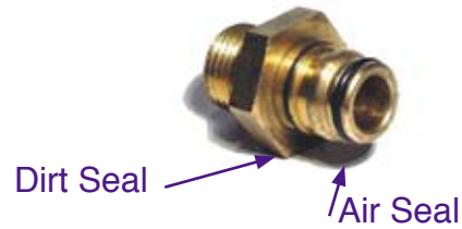
Male Connector
