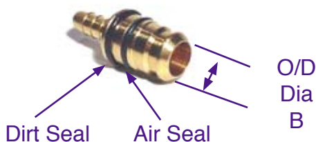
Straight Connector
