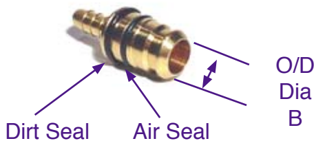
Straight Connector
