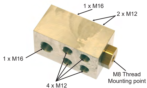
8 Port Aluminium Manifold Valve c/w Plug Part No. 7994
