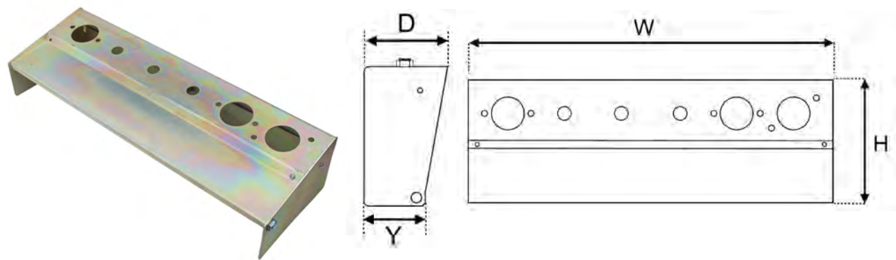
Slim-Line 3 Line Coupling Box
