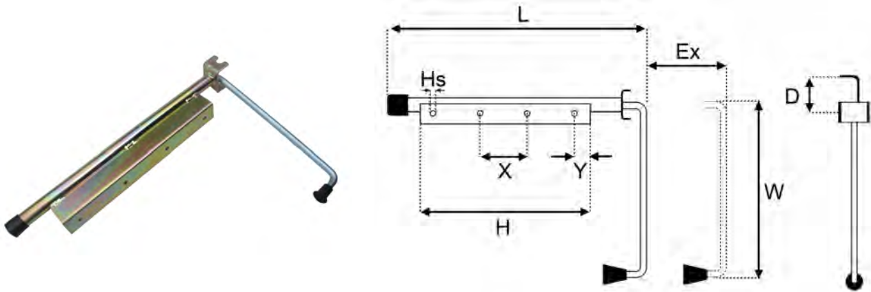
Spring Loaded Door Retainer
